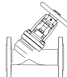
▶ 069plus – Y-pattern with flanges and bellows seal
