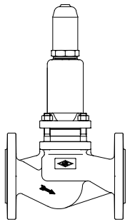
▶ 750 Pressure regulating valve, straight through with flanges – spring loaded
