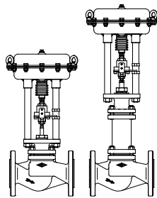
▶ 405/460 Stop valve with pneumatic actuator DP 32 - 35
