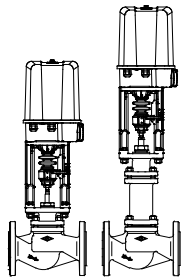
▶ 405/460 Stop valve with electric actuator Premio 2,2 kN - 15 kN
