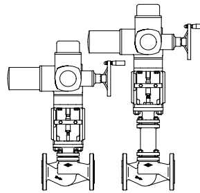
▶ 405/460 Stop valve with electric actuator AUMA SA 07.2 - 16.2
