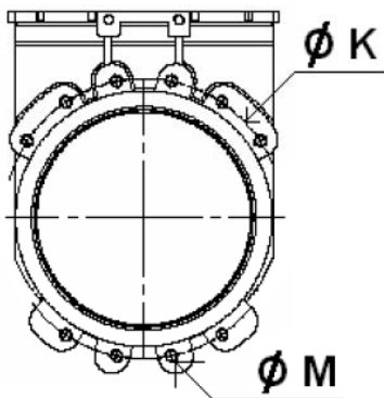
DN 350 – 400
