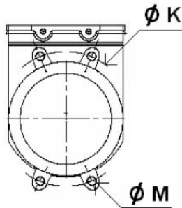
DN 80 – 200
