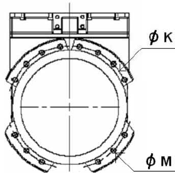
DN 450 – 600
