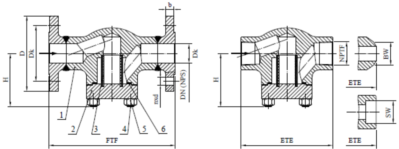
Drawing C.3.1 Parts and dimensions
