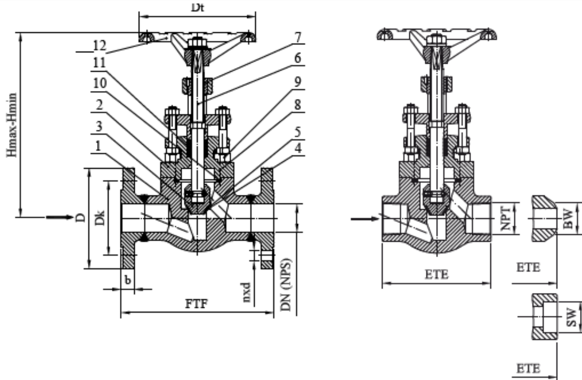
Drawing A.7.1 Parts and dimensions
