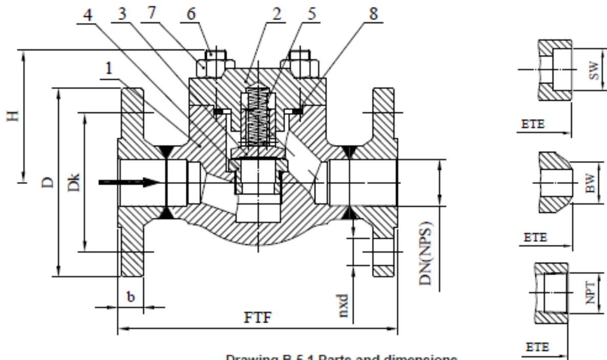
Drawing B.5.1 Parts and dimensions
