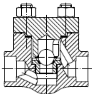
Forged Ball Check Valve
