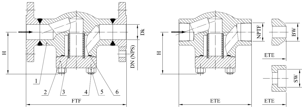
Drawing C.3.1 Parts and dimensions
