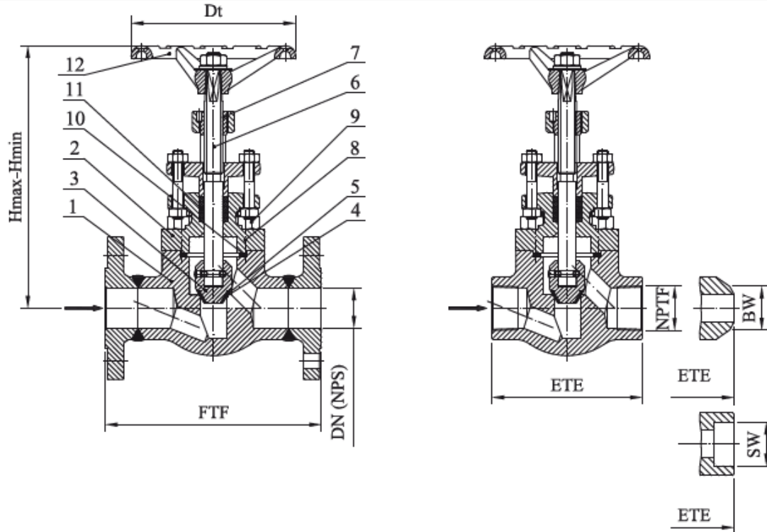
Drawing A.7.1 Parts and dimensions
