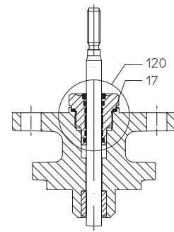
I. EPDM-sealing
