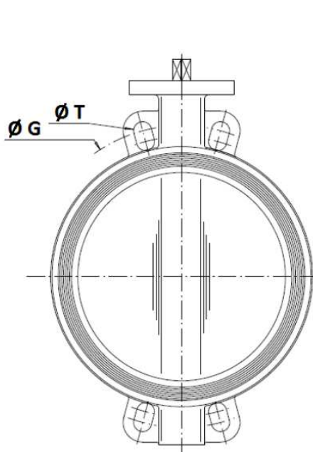
DN250 – 400
