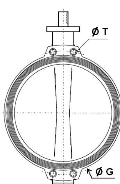
DN450-1400
