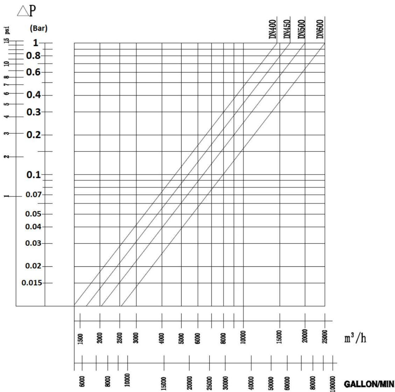
HEAD LOSS GRAPH DN400-600 :
