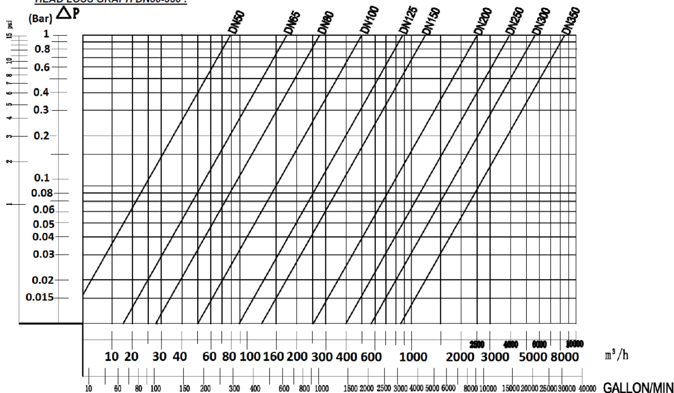
HEAD LOSS GRAPH DN50-350 :
