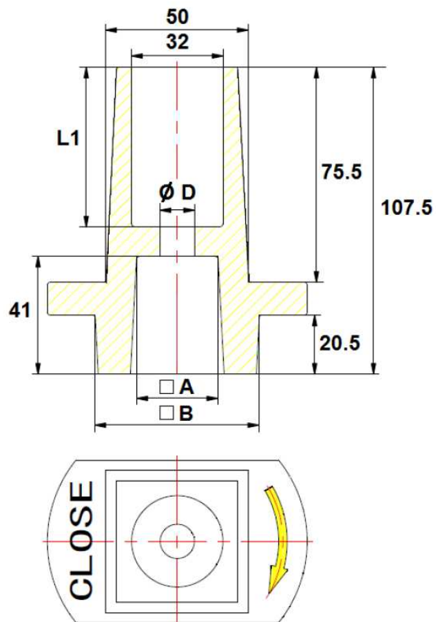
DN 350 - 400
