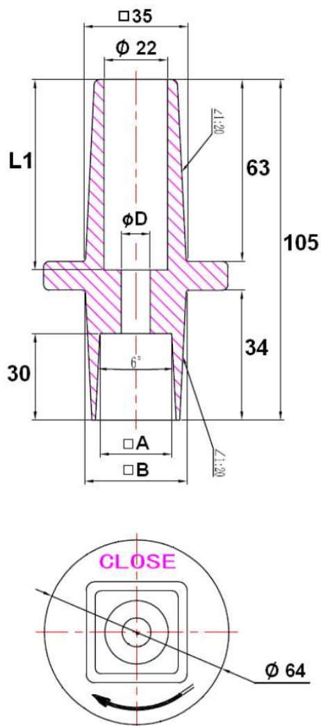
DN 40 – 300
