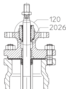
III. Stainless steel bellows seal with EPDM-sealing
