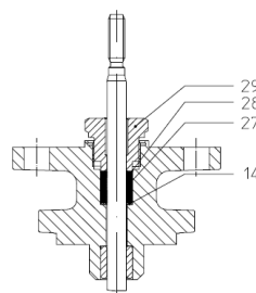
II. PTFE- / pure graphite-packing
