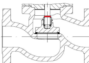
DN65-100: Back seat (when fully opened valve) DN10-50: standard
