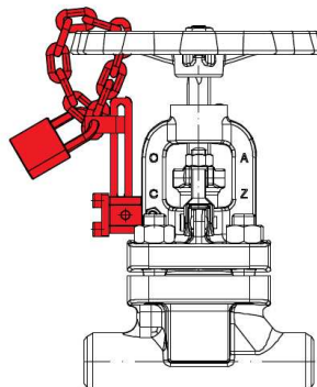
Tamper resistant handwheel blocking
