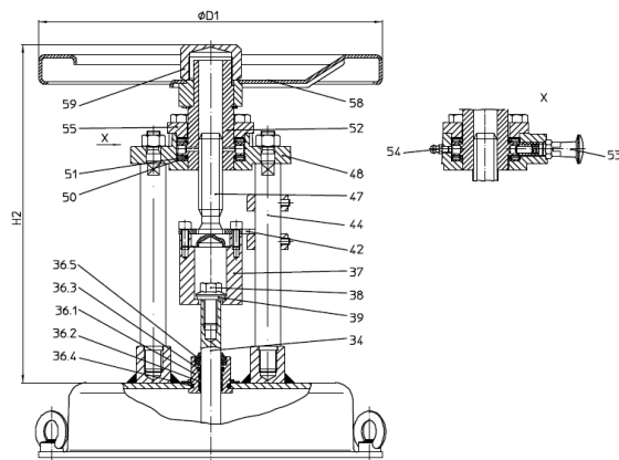
DP30 / DP32 / DP33 / DP34 Top mounted handwheel
