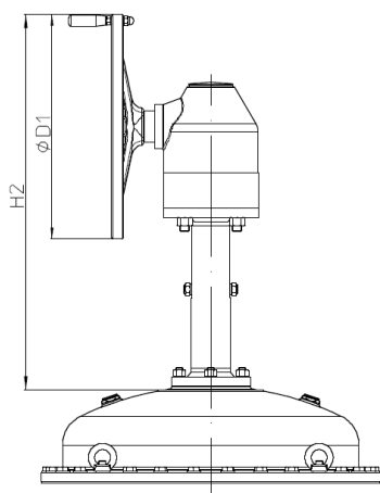
DP35 Top mounted handwheel with bevel gear
