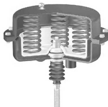
DP-Actuator Extended stem on air failure
