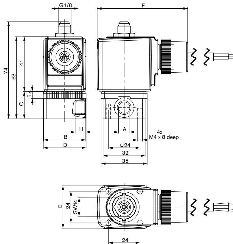
Threaded version
