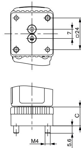
Flange version (SFB)
