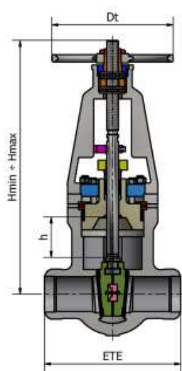
GHP with welding ends - CAST
