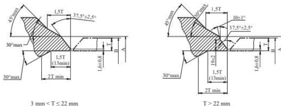
Figure A.13 - Form of the butt welding ends
