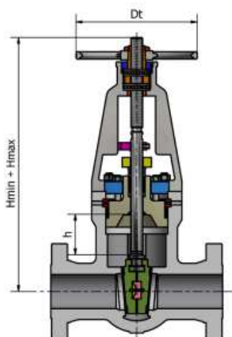
GHP with flanged ends - CAST
