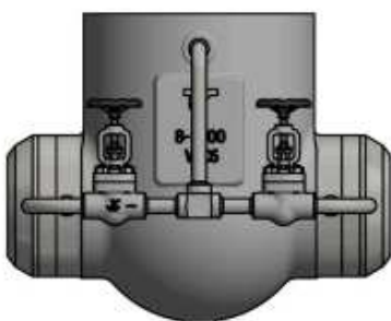
Figure A.8 With double by-pass & equalizing pipe
