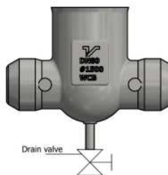
Figure A.6 With drain valve
