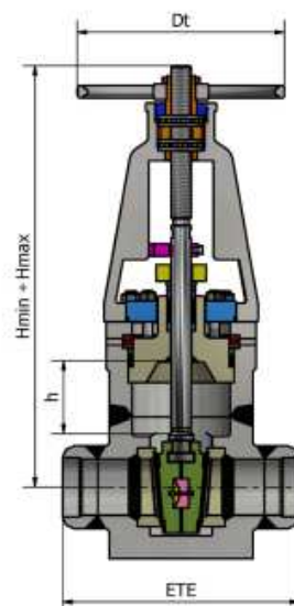
GHP with welding ends - FORGED
