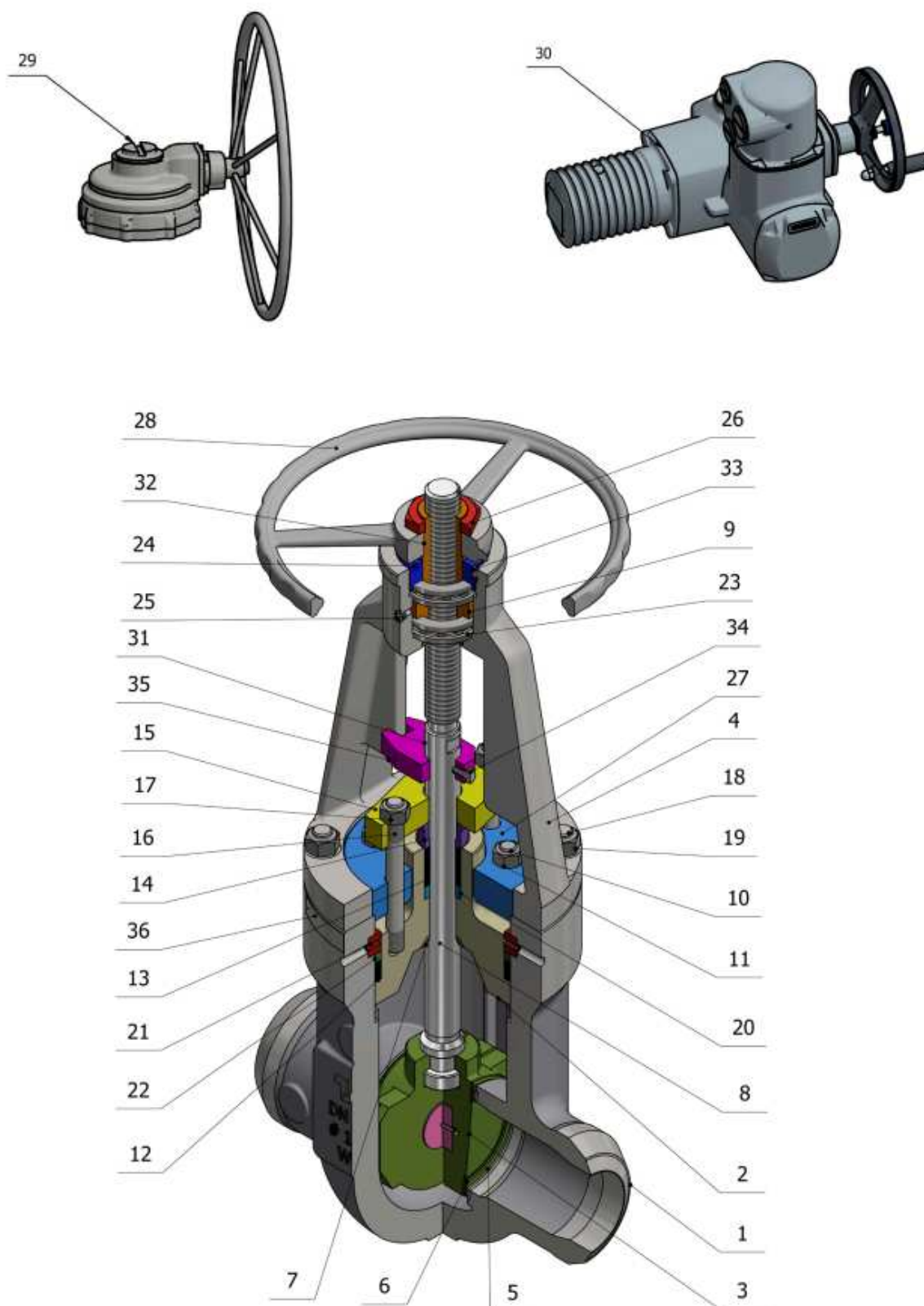
Figure A.1 Parts
