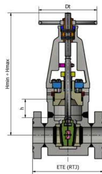
GHP with flanged ends - FORGED
