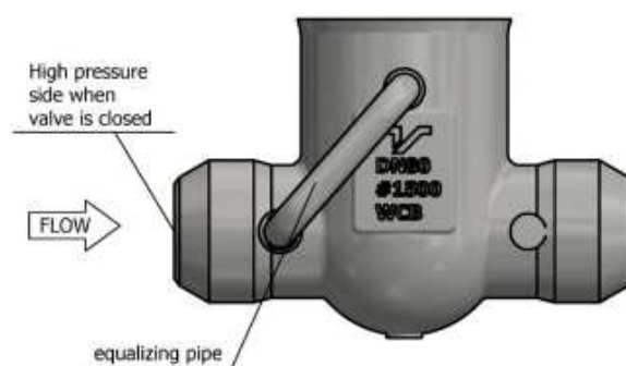
Figure A.4 With equalizing pipe
