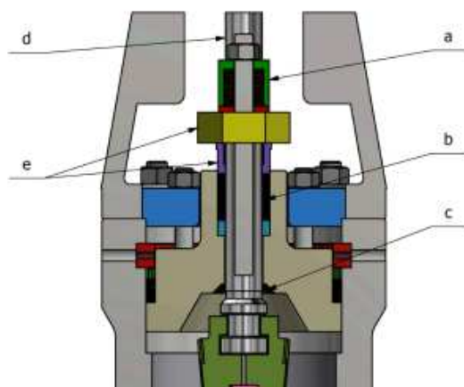
Figure A.12 Stem seal
